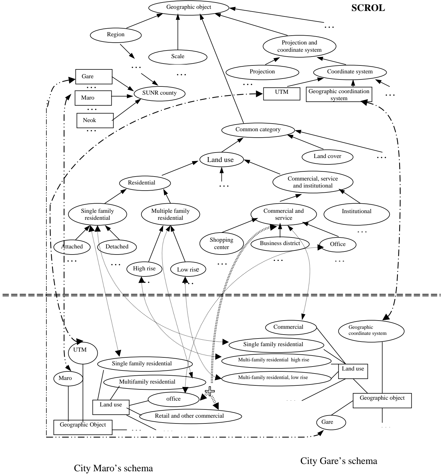
Figure 2 An example of SCROL , local schema and Ontology mapping
