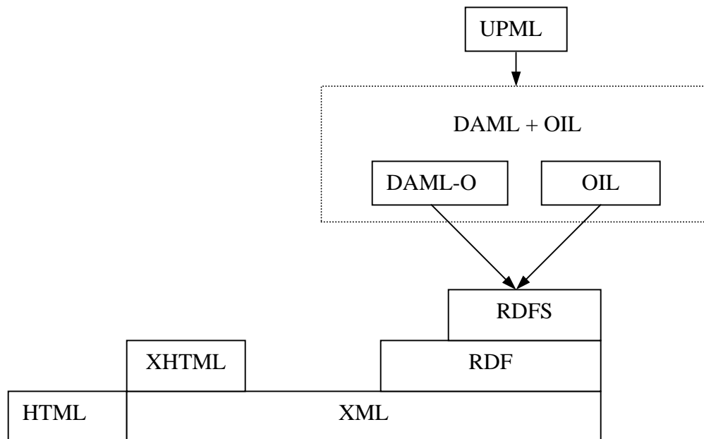
Figure 1 Layer Language model for the WWW (Fensel, Hendler et al., 2002)
