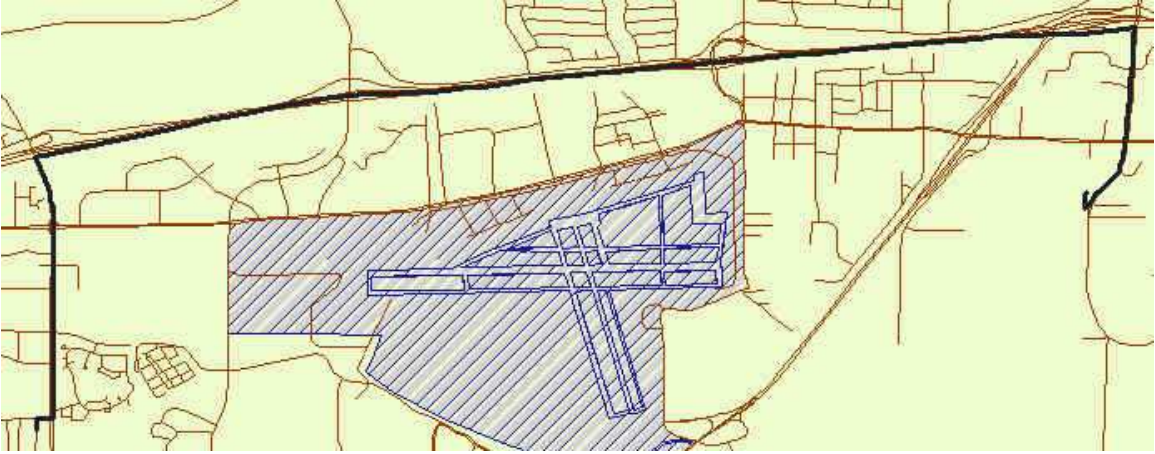
Figure 6: Map matching result after Dempster belief test with multi-criterion fusion.
